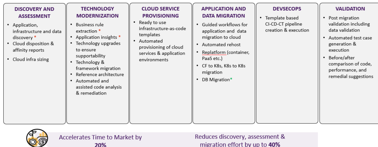
Figure 3. Infosys Cloud Application Modernisation Platform (iLEAD)
