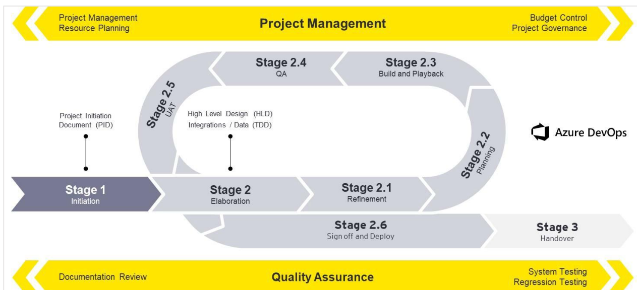
Figure 3 - Agile Methodology
