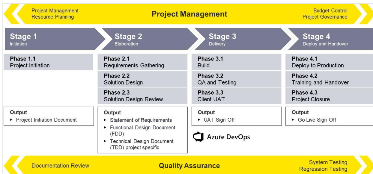
Figure 3 - Waterfall Methodology
