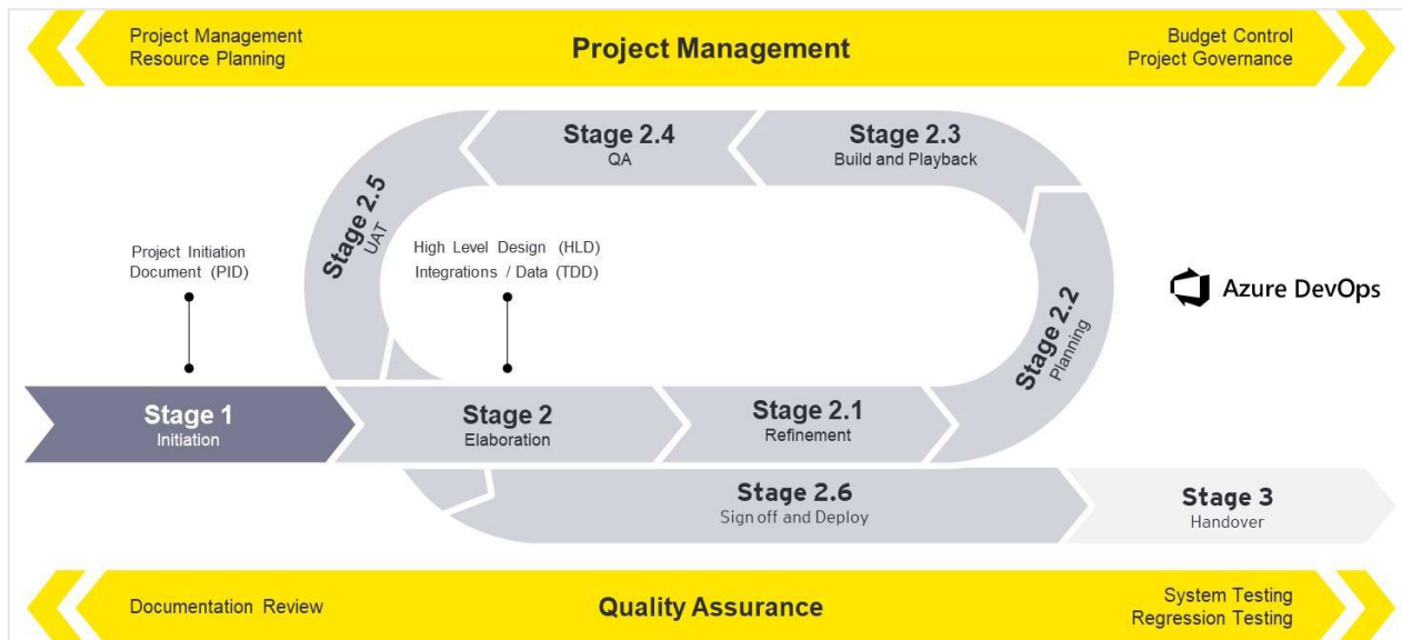
Figure 4 - Agile Methodology
