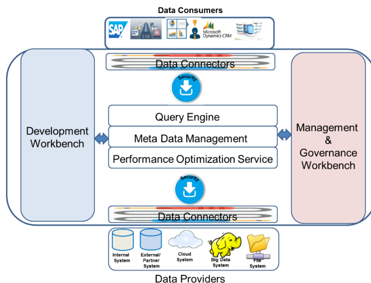
Figure 1: Reference model for data virtualisation
