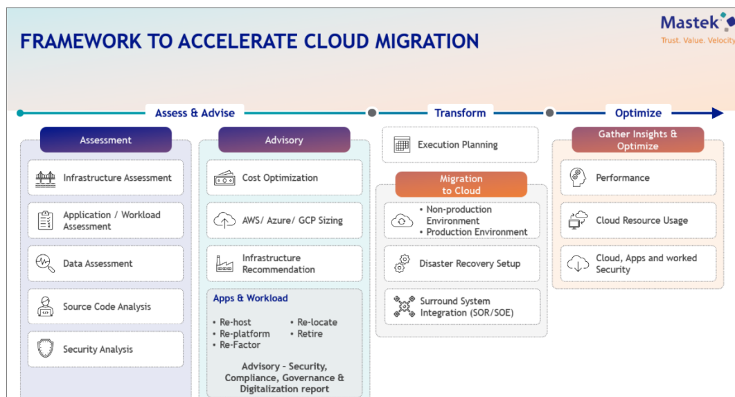
Figure 2: Migration Framework
