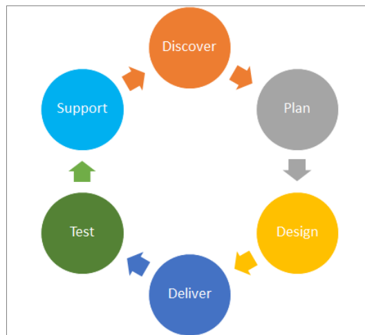
Figure 1: Process Cycle
