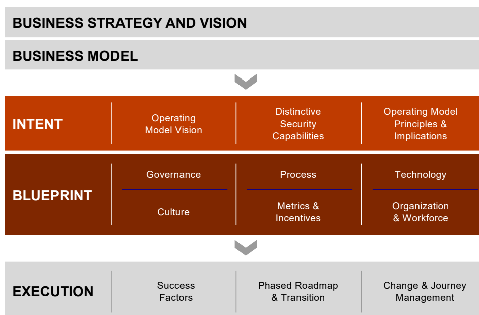
Figure 2: Transformation Methodology
