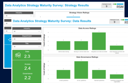
Maturity Scoring
