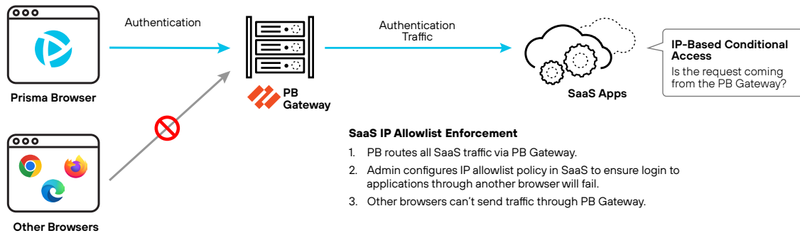
Figure 3. Enforcing IP-based IdP conditional access to business applications via PB Gateway
