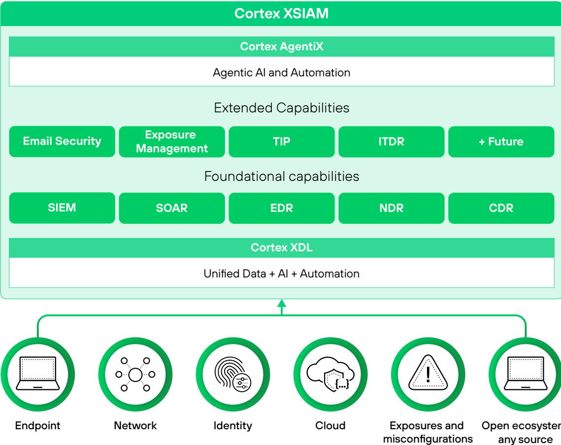
Figure 1. Cortex XSIAM core and advanced capabilities
