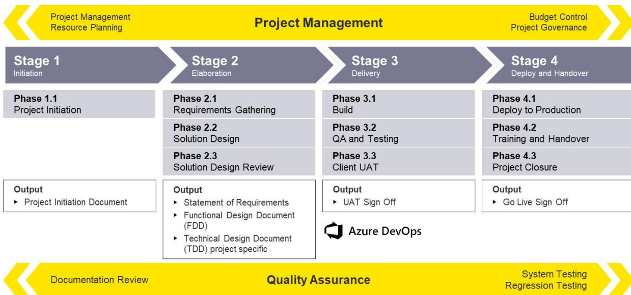
Figure 4 - Waterfall Methodology
