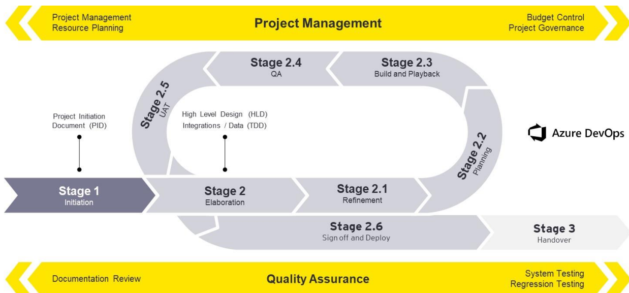
Figure 5 - Agile Methodology
